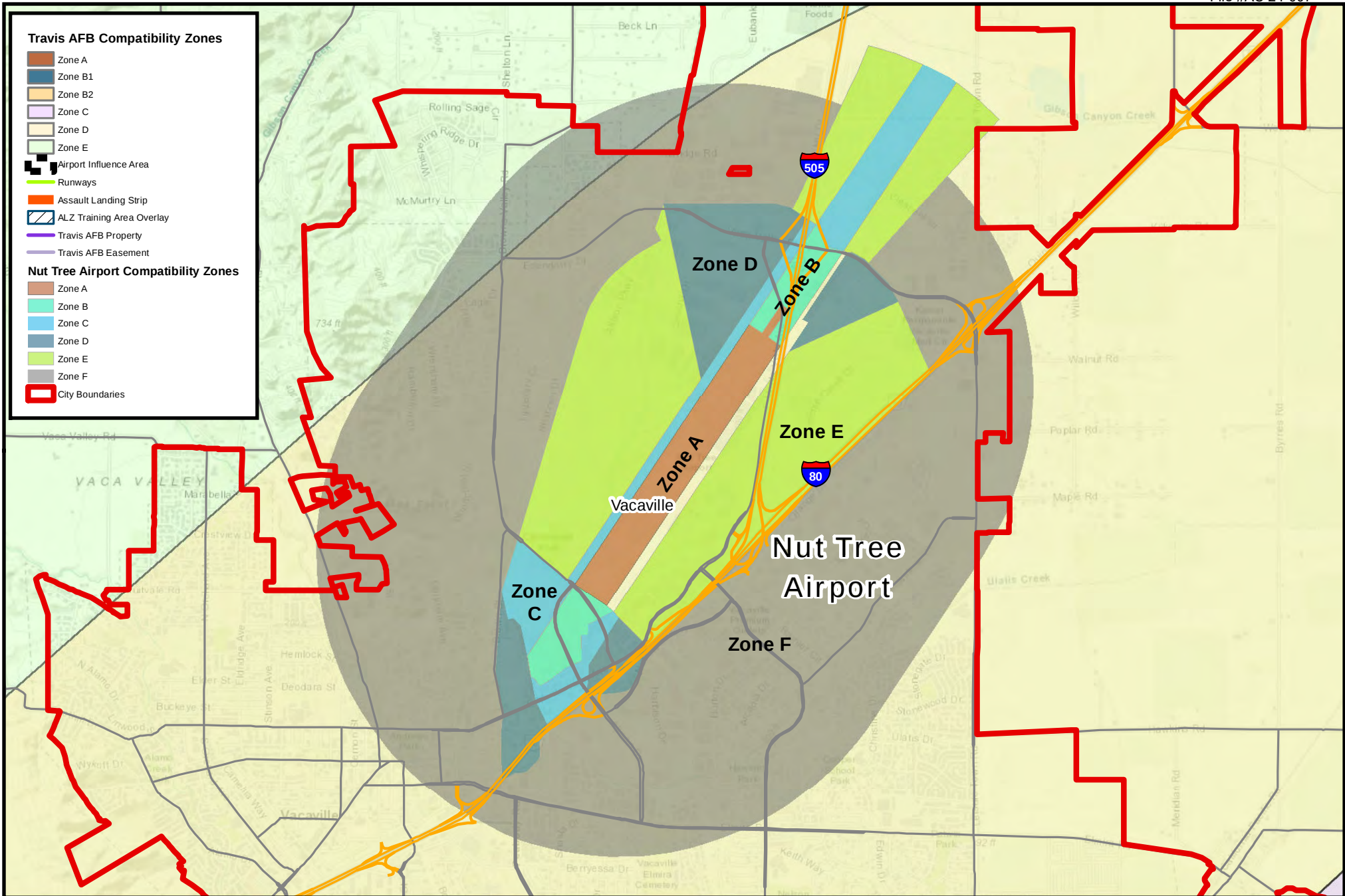
Airport Compatibility Zones & Travis AFB Influence Area
