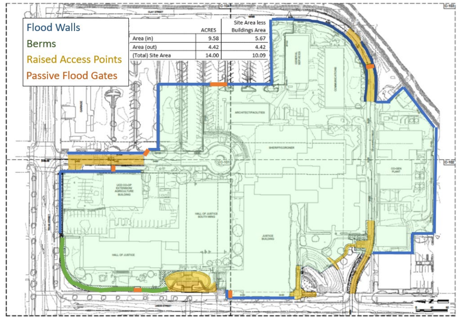
Asset Protection Campus Site Plan
