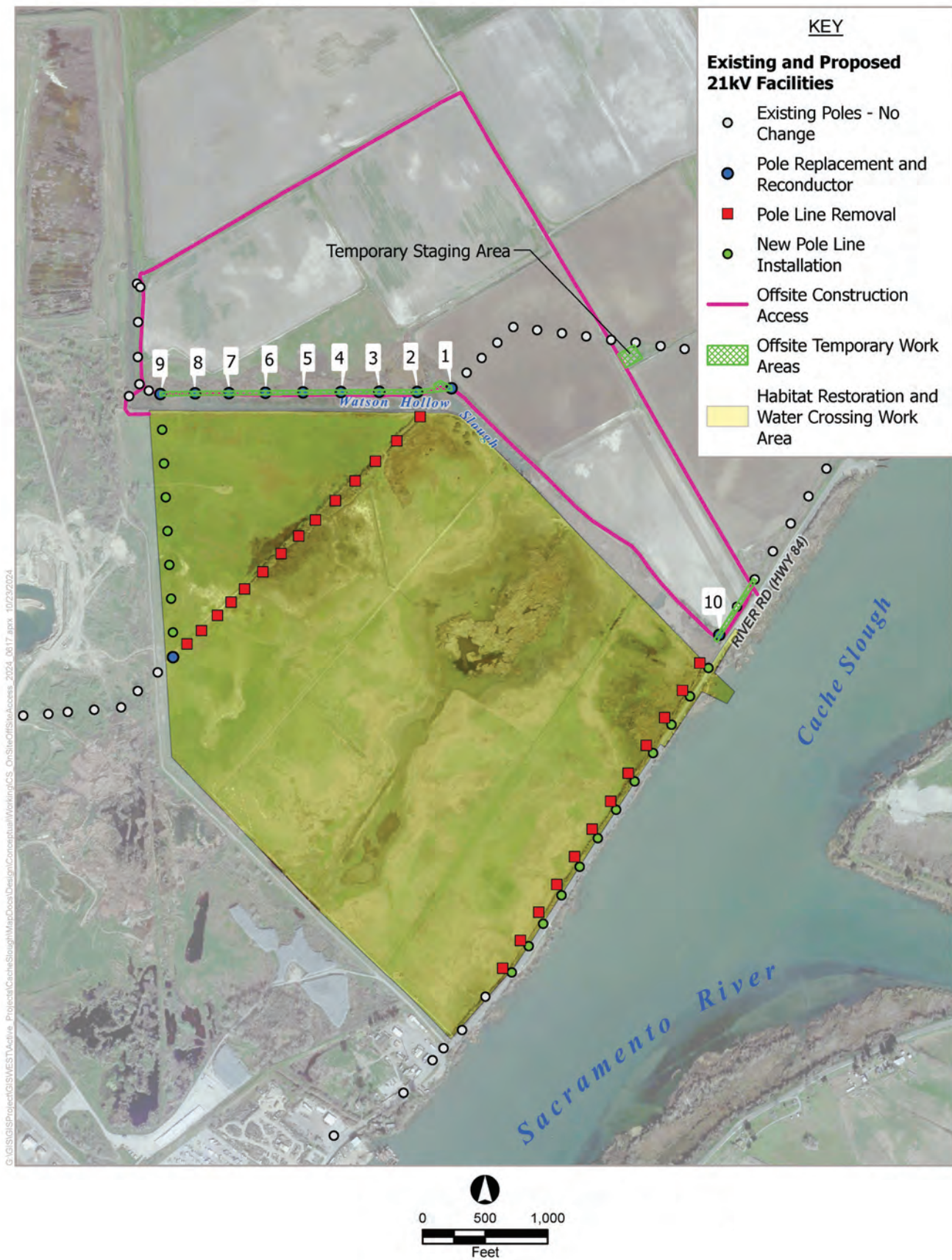
Figure 1-4 Onsite and Offsite Utility Infrastructure Improvements
