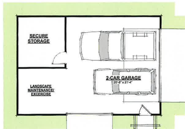
DETACHED GARAGE PLAN (704 S.F.)
