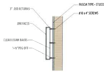
Typical Non Illuminated Reverse pan channel letters / logo
