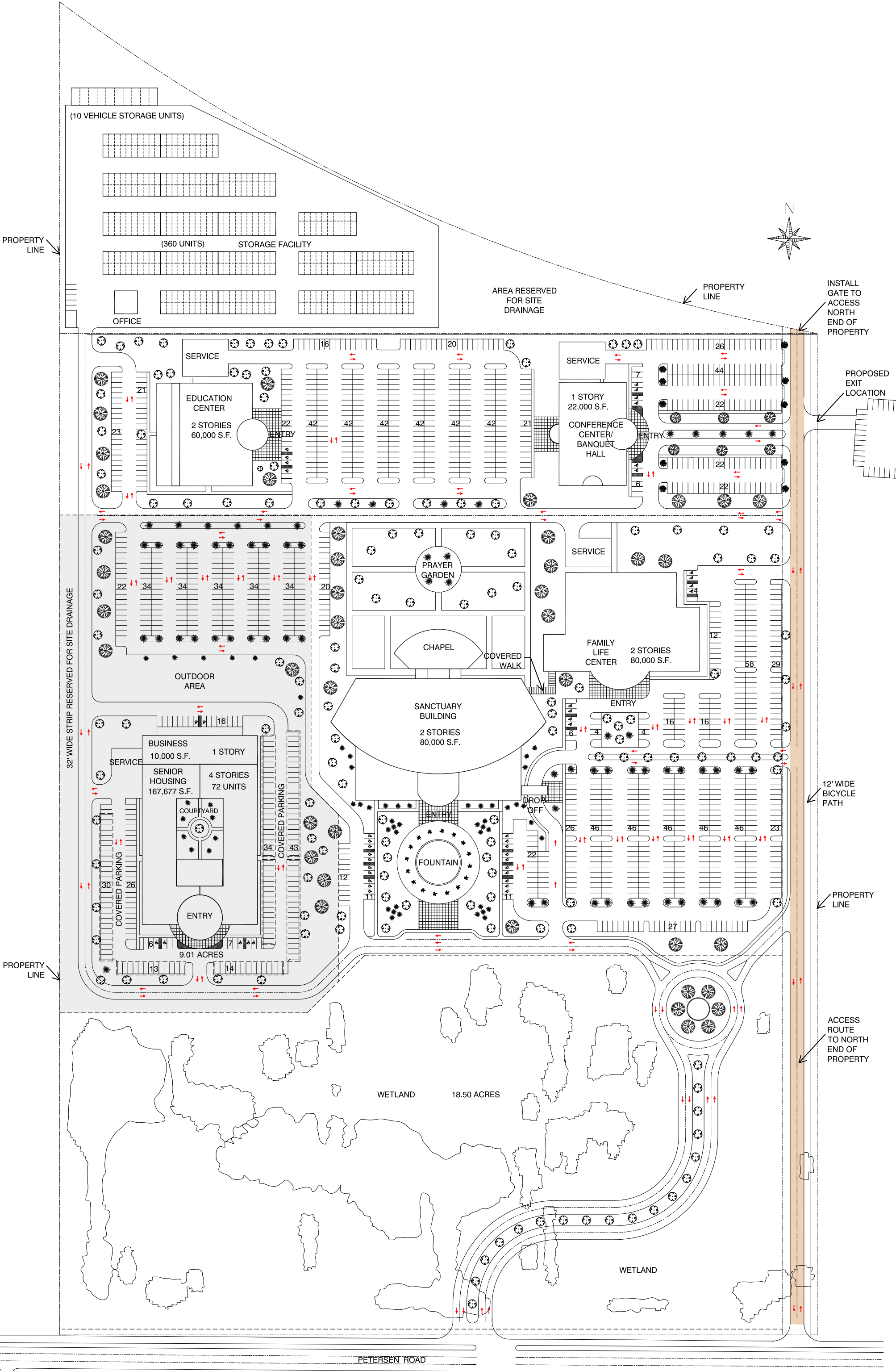
SITE PLAN
