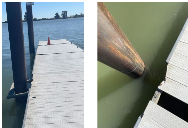
Figure 2/3 Damage and destruction of brackets for anchor pilings
